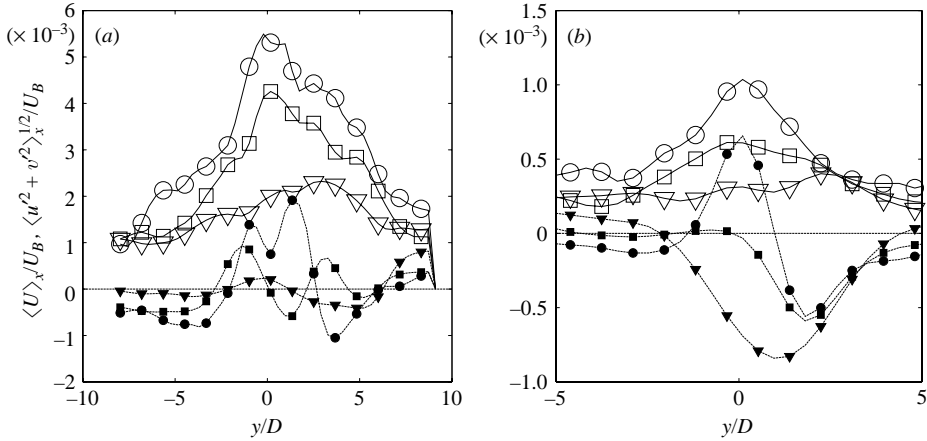
FIGURE 11. Profile of mean velocity (filled symbols) and quadratic fluctuations (open symbols) at times Nt = 50 ( \circ ), Nt = 100 ( \square ) and Nt = 300 ( \nabla ) for (a) a cylinder with F = 25 and Re = 27000 , (b) a spheroid with F = 40 and Re = 25000 .
